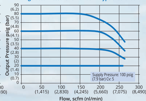
Regulated Pressure vs Flow: 3/4" Type 6100/6200
