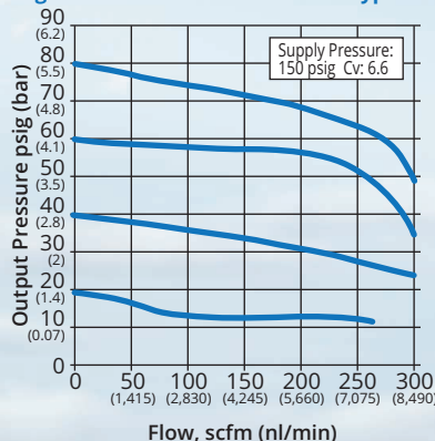
Regulated Pressure vs Flow: 1/2" Type 6000
