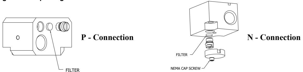
Figure 3 – Replacing Filter
