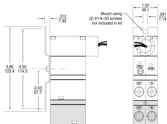
Figure 2 - Panel Mounting
