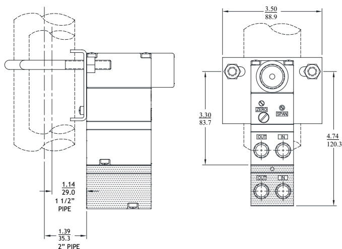
Figure 1 - Pipe Mounting
